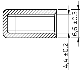
sectional drawing A-A
