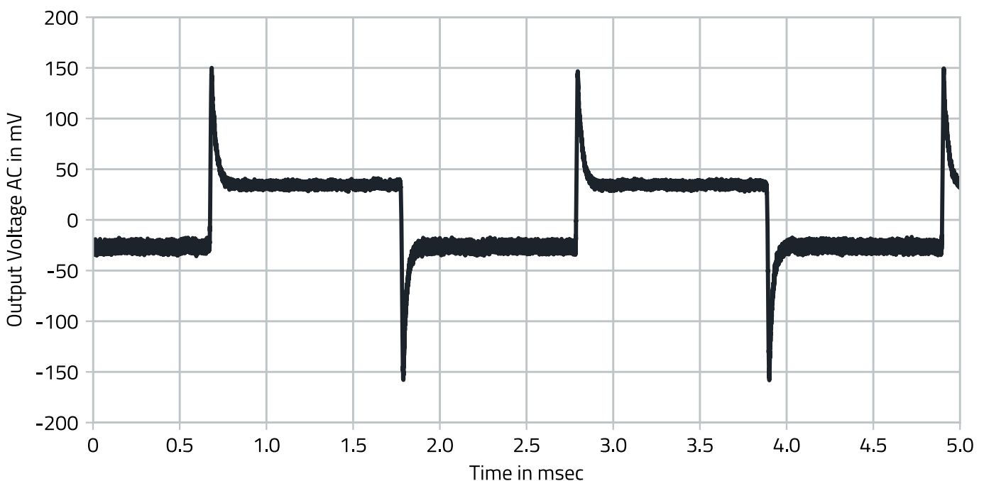
Figure 20: 171023802 V IN = 24V, V OUT = 5V, C OUT = 47μF, load jumps 10% - 100%.
