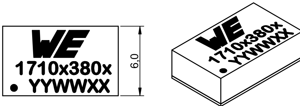
Figure 31: Physical dimensions.
