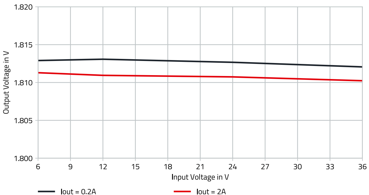
Figure 13: 171023802 Line Regulation V_{OUT} = 1.8V .
