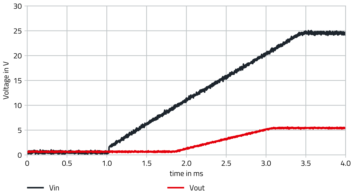
Figure 26: 171023802 soft start V_{IN} = 24V , V_{OUT} = 5V , T_A = 25^\circ C .
