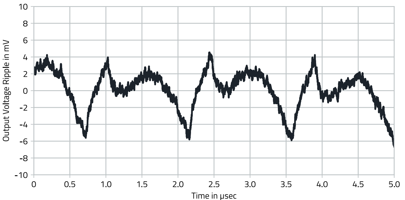
Figure 22: 171023802 output voltage ripple V_{IN} = 24V , V_{OUT} = 5V , I_{OUT} = 2A , C_{OUT} = 47\mu F .
