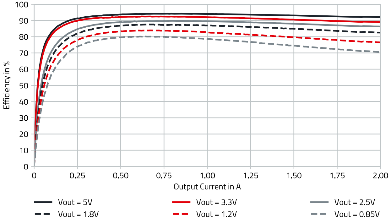
Figure 6: 171023802 efficiency V IN = 12V.
