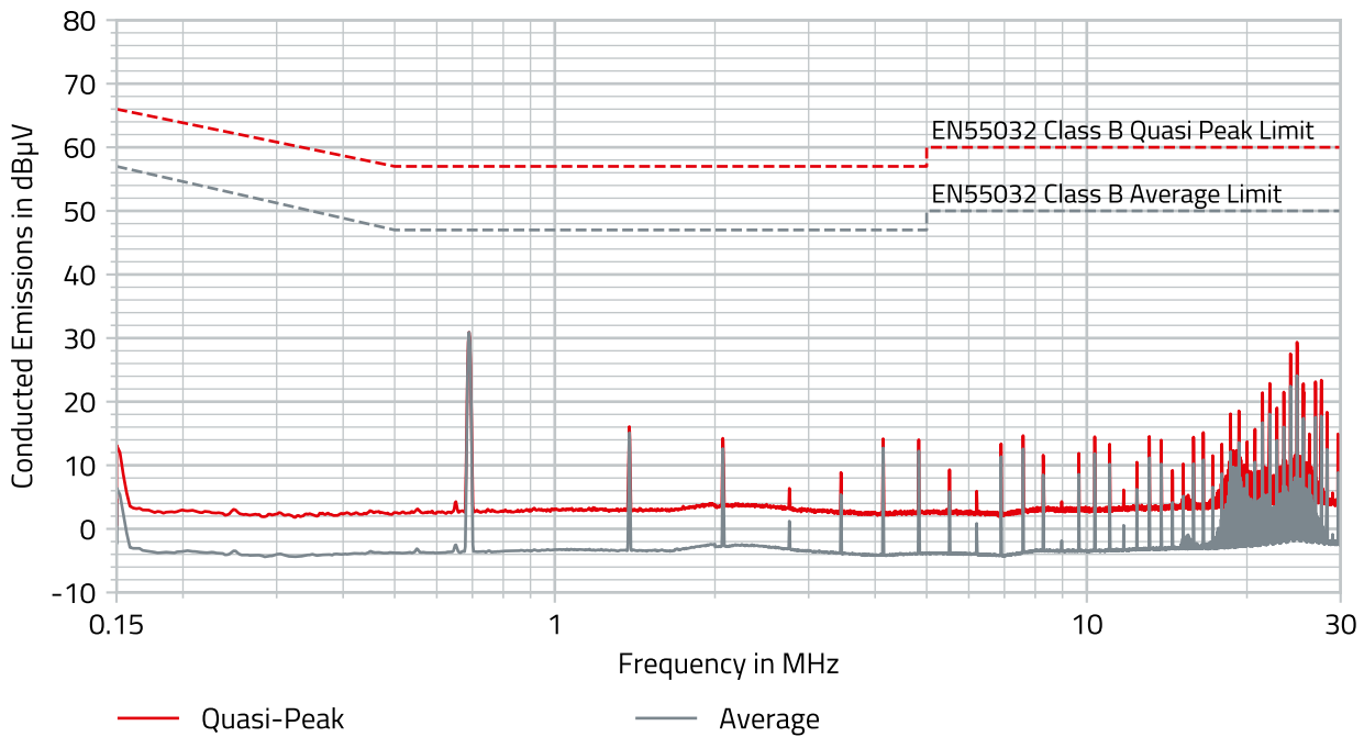
Figure 4: Conducted emissions (fixed frequency) 171023802 V_{IN} = 24V , V_{OUT} = 5V , I_{LOAD} = 2A with input filter.
