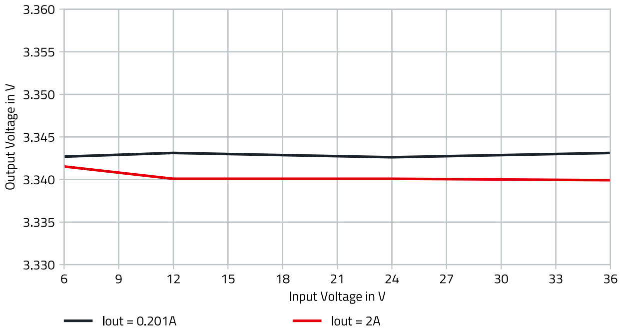
Figure 14: 171023802 Line Regulation V OUT = 3.3V.
