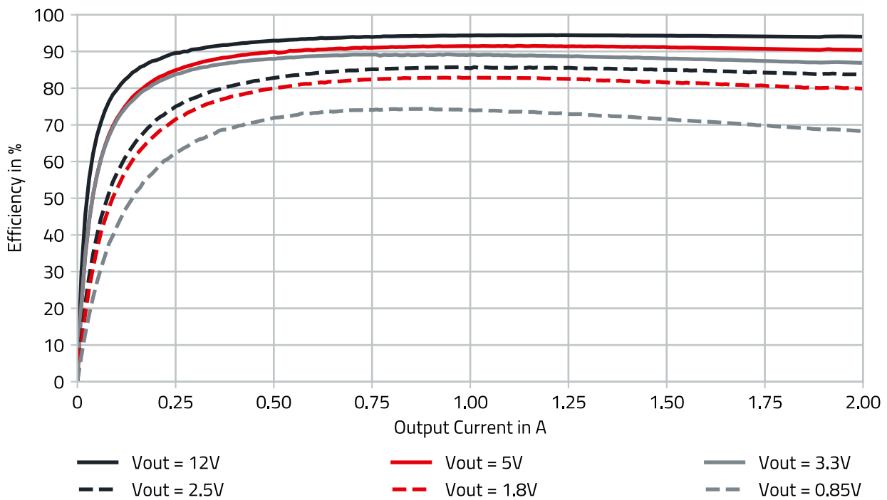
Figure 7: 171023802 efficiency V IN = 24V.
