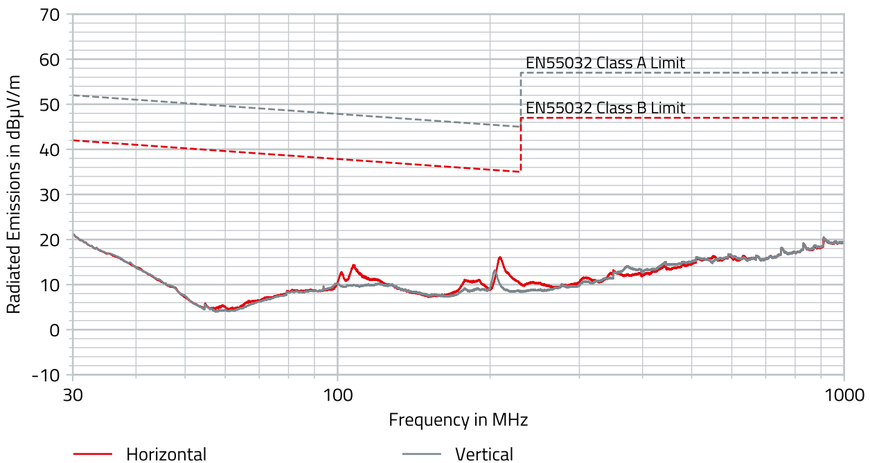
Figure 3: Radiated emissions (spread spectrum) 171023802 (3m antenna distance) V_{IN} = 24V , V_{OUT} = 5V , I_{LOAD} = 2A with input filter.
