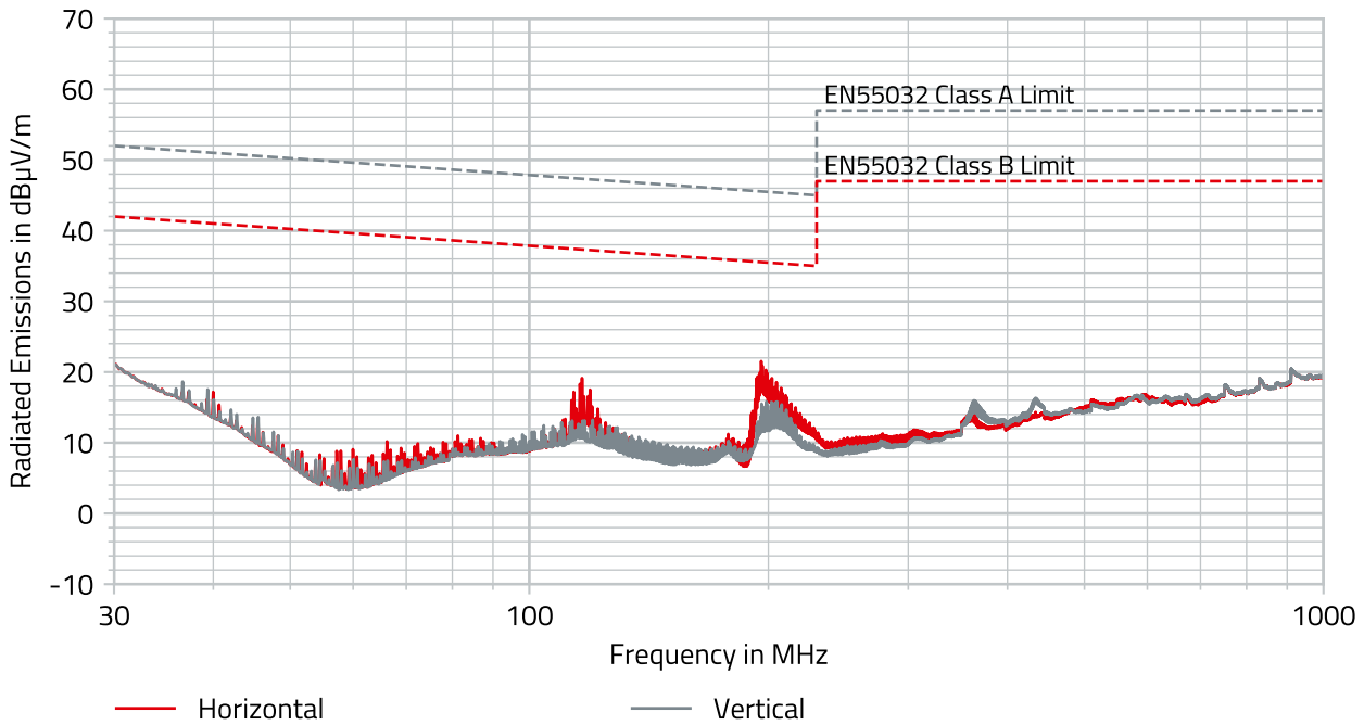
Figure 2: Radiated emissions (fixed frequency) 171023802 (3m antenna distance) V_{IN} = 24V , V_{OUT} = 5V , I_{LOAD} = 2A with input filter.
