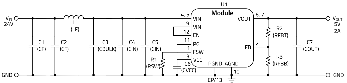
Figure 29: 171023802 design example schematic.
