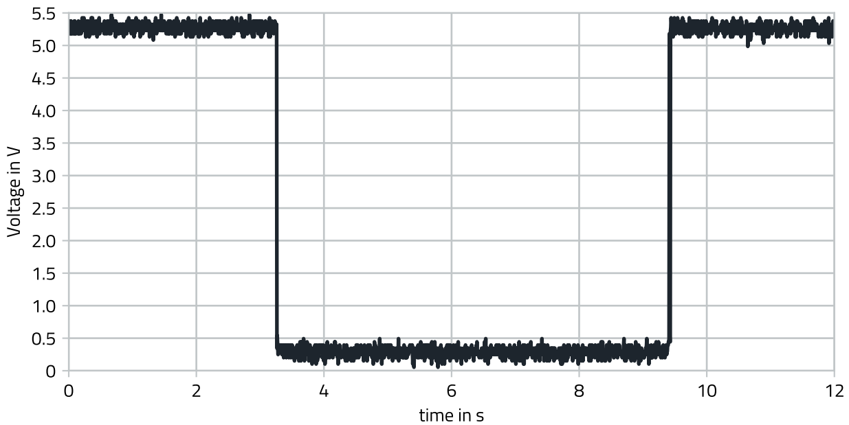
Figure 25: 171023802 short circuit protection V_{IN} = 24V , V_{OUT} = 5V .
