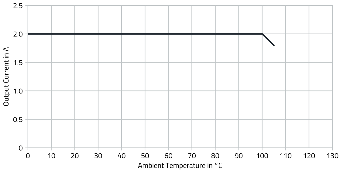
Figure 9: 171023802 output current thermal derating V_{IN} = 24V , V_{OUT} = 5V .
