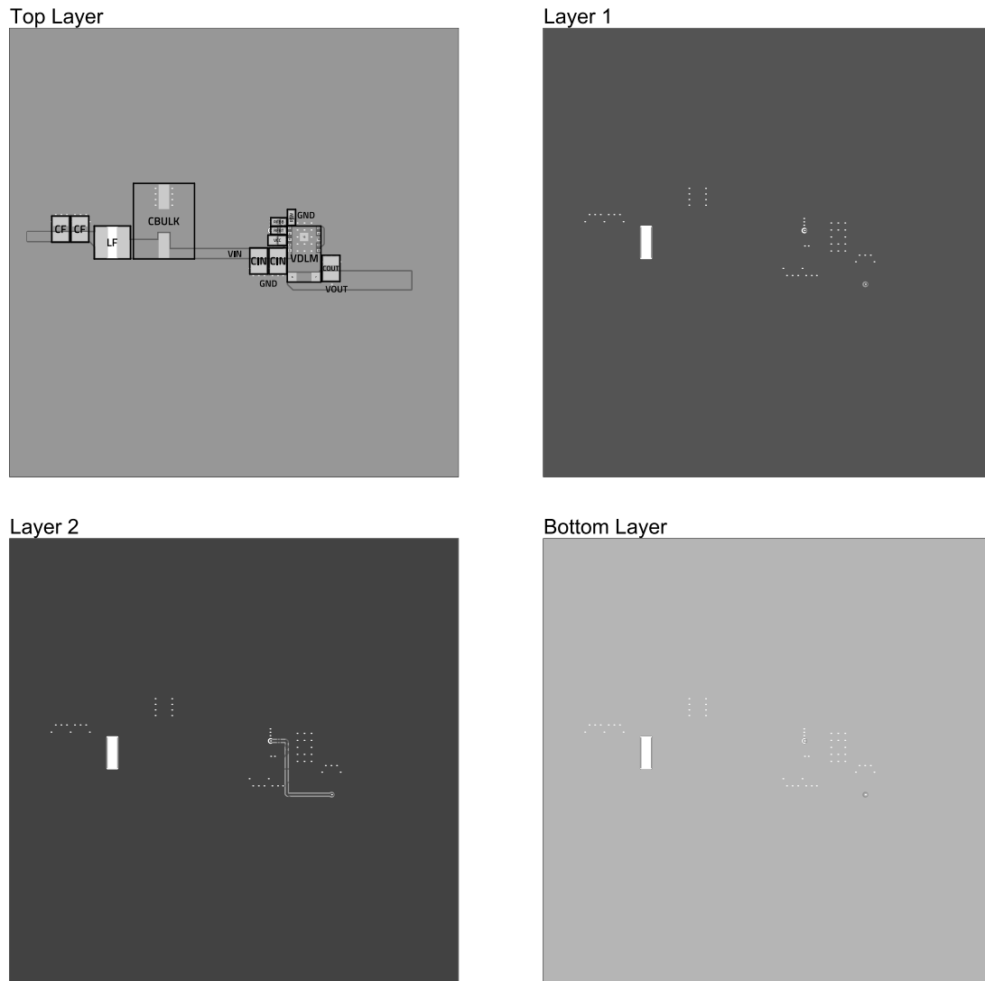
Figure 28: 171023802 layout recommendation.
