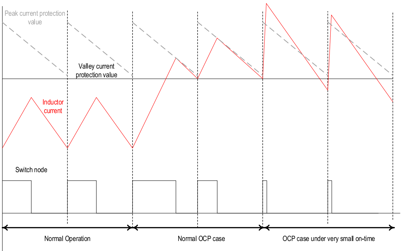
Figure 23: 171023802 overcurrent protection inductor current.
