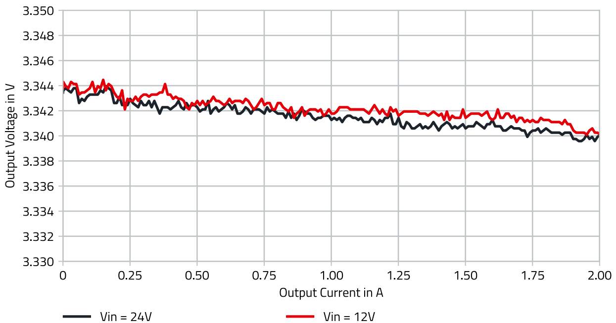
Figure 11: 171023802 Load Regulation V_{OUT} = 3.3V .
