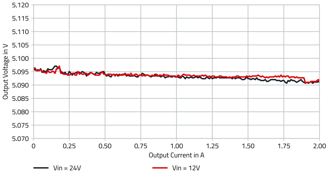
Figure 12: 171023802 Load Regulation V_{OUT} = 5V .
