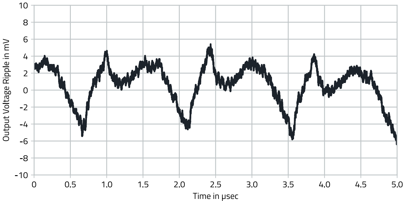
Figure 21: 171023802 output voltage ripple V_{IN} = 24V , V_{OUT} = 5V , I_{OUT} = 200mA , C_{OUT} = 47\mu F .
