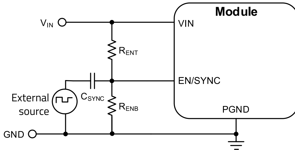
Figure 27: 171023802 sync to external signal schematic.
