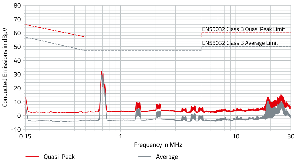
Figure 5: Conducted emissions (spread spectrum) 171023802 V_{IN} = 24V , V_{OUT} = 5V , I_{LOAD} = 2A with input filter.
