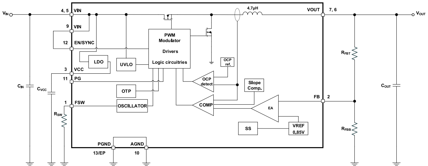
Figure 17: 171023802 block diagram.
