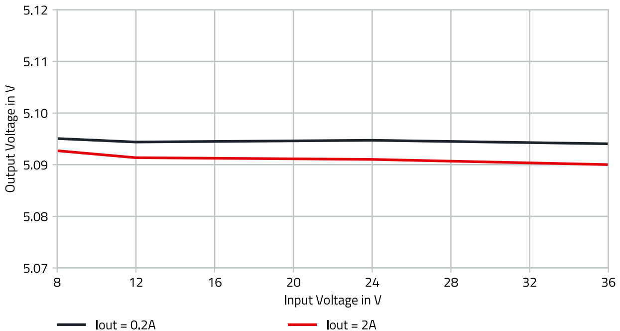
Figure 15: 171023802 Line Regulation V OUT = 5V.
