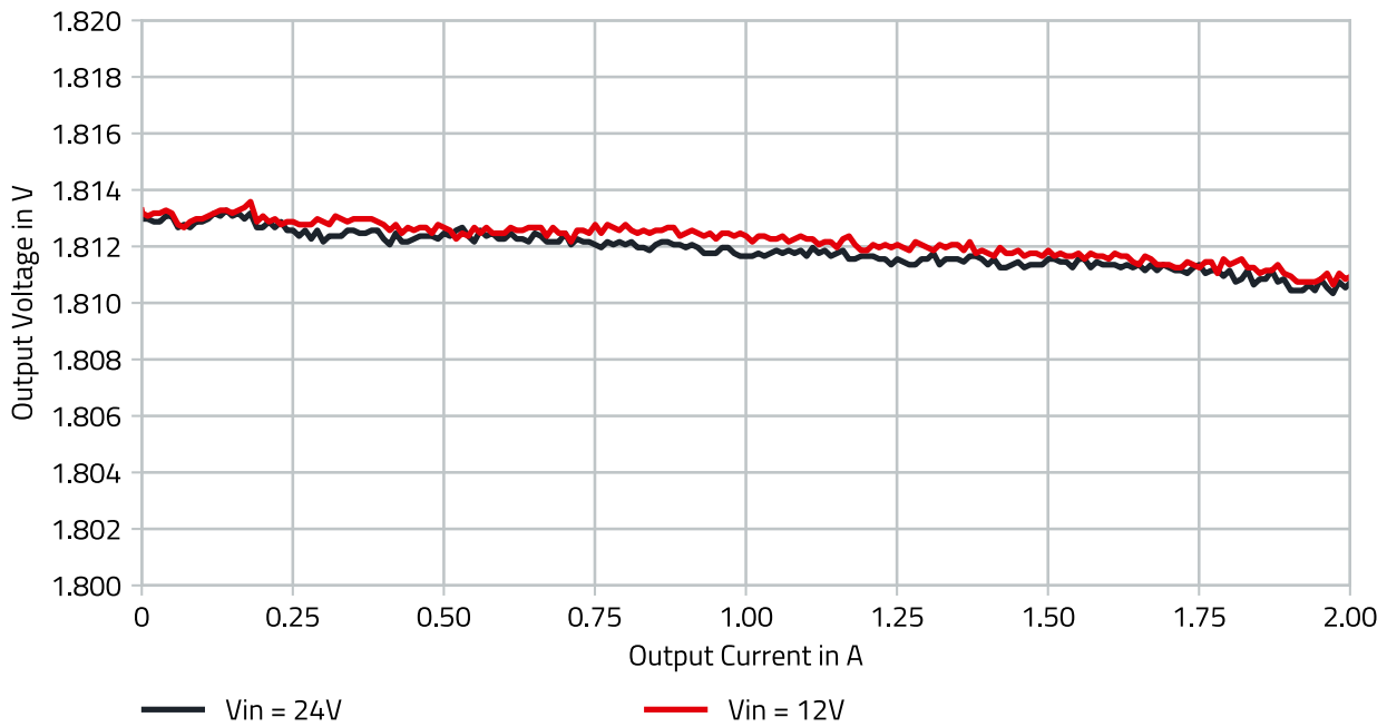
Figure 10: 171023802 Load Regulation V_{OUT} = 1.8V .
