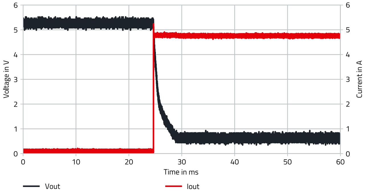
Figure 24: 171023802 overcurrent protection V_{IN} = 24V , V_{OUT} = 5V , I_{OUT} = 0A to 4.8A .
