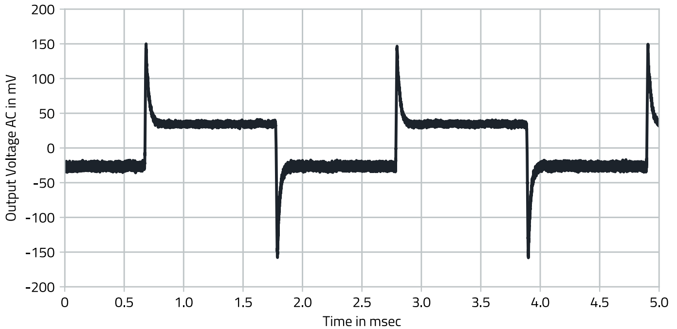
Figure 16: 171023802 V_{IN} = 24V , V_{OUT} = 5V , C_{OUT} = 47\mu F , load jumps 10% - 100%.
