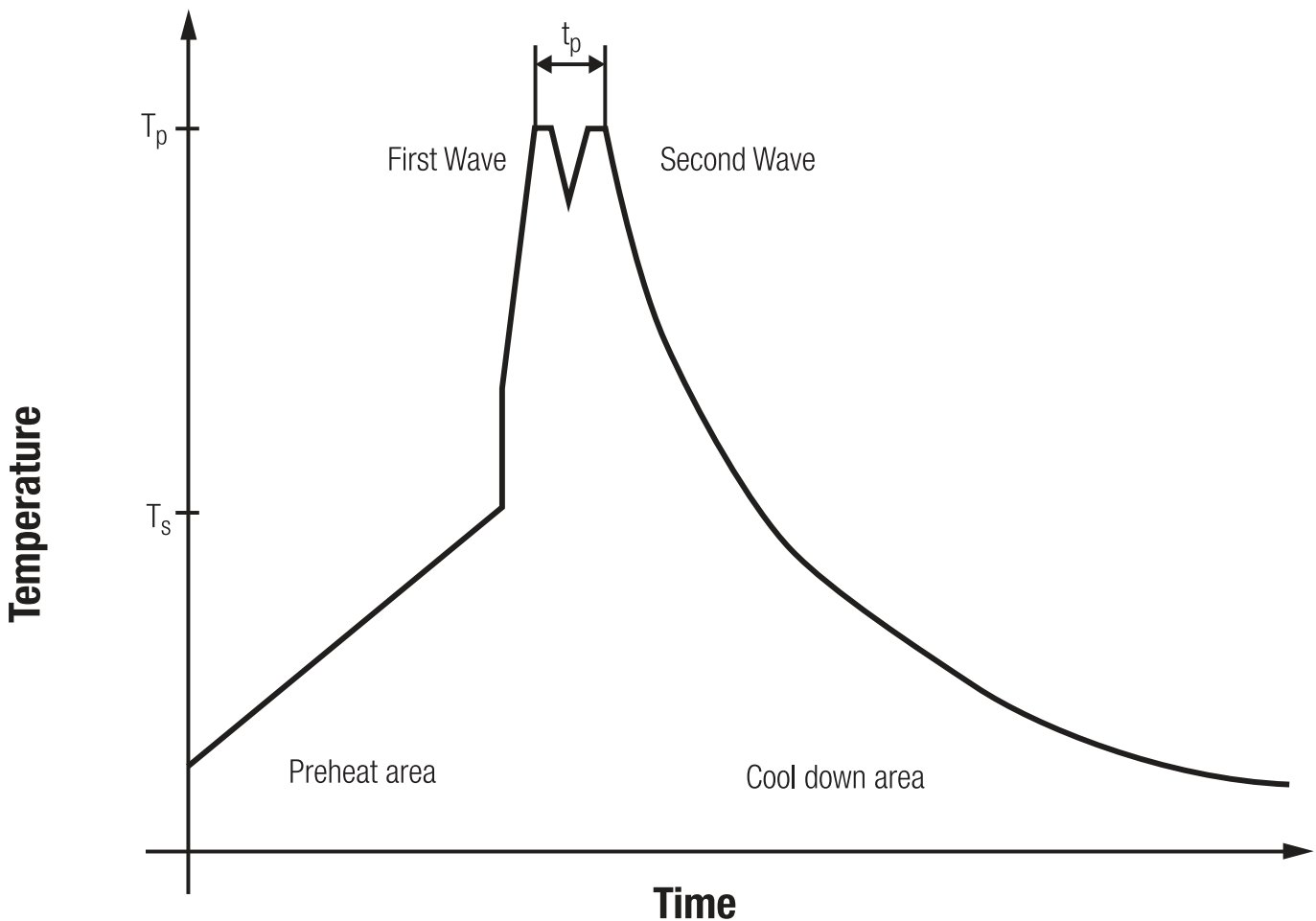
Figure 17: Solder profile.
