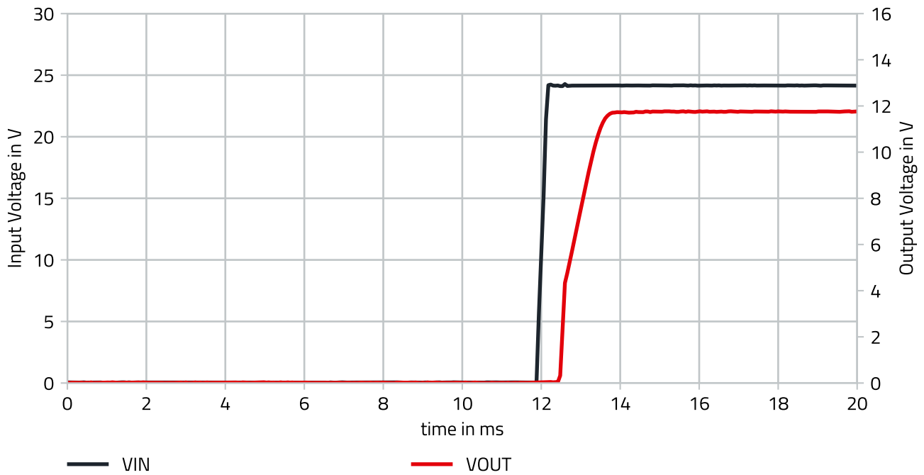
Figure 10: Soft-start, V_{IN} = 24V , V_{OUT} = 12V , I_{OUT} = 2A .
