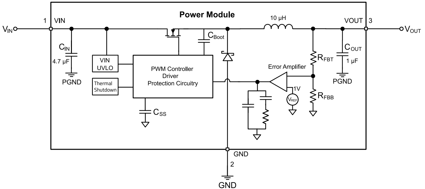
Figure 8: 173021236 block diagram.
