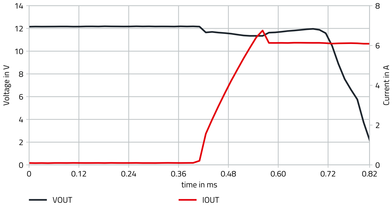
Figure 12: Over current protection, V_{IN} = 24V , V_{OUT} = 12V , I_{OUT} = 2A .
