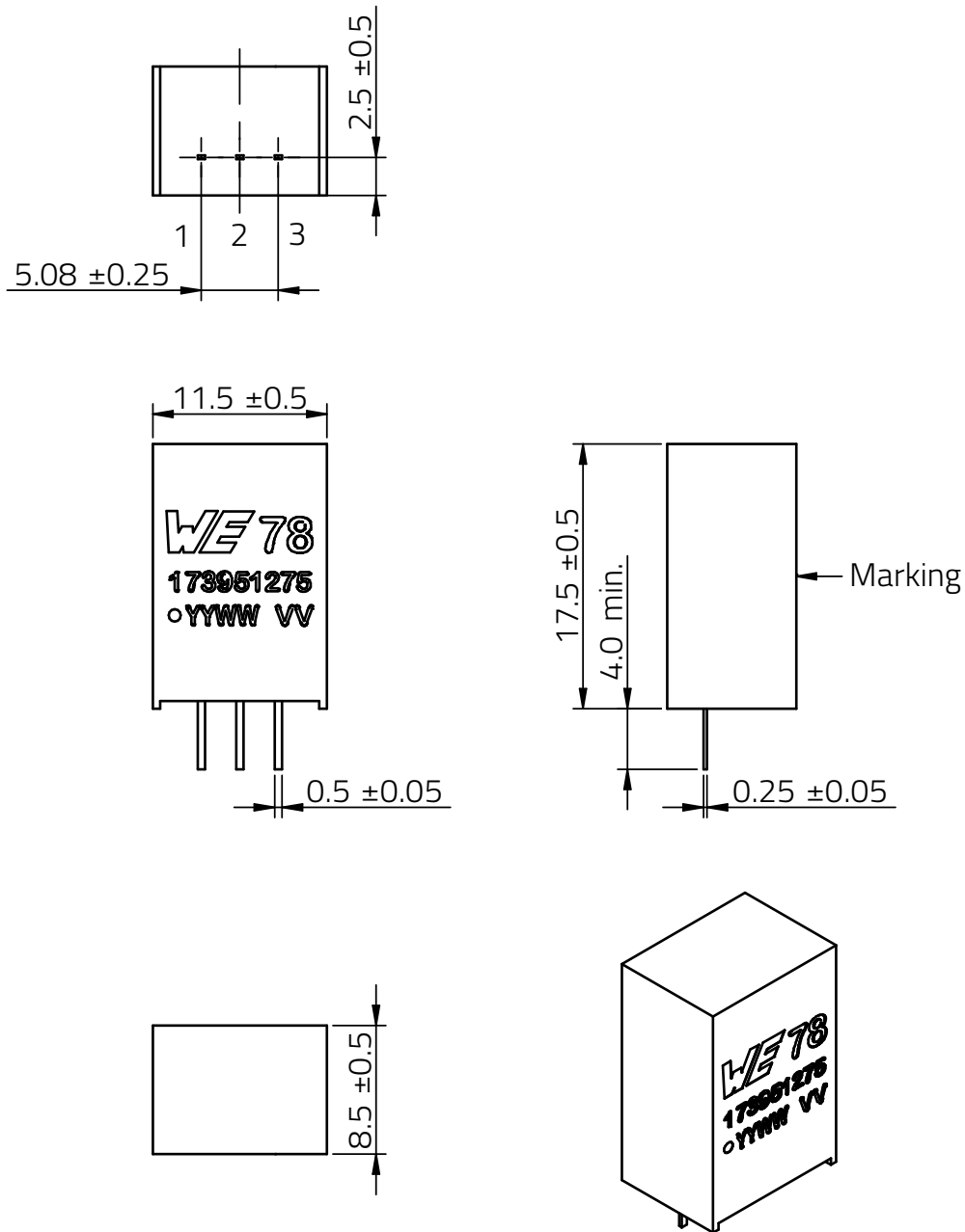
Figure 17: Physical dimensions.
