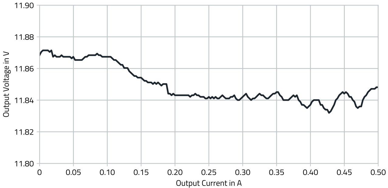
Figure 6: Load regulation.
