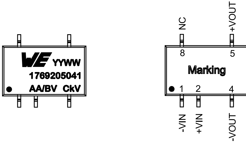
Figure 1: Pinout.
