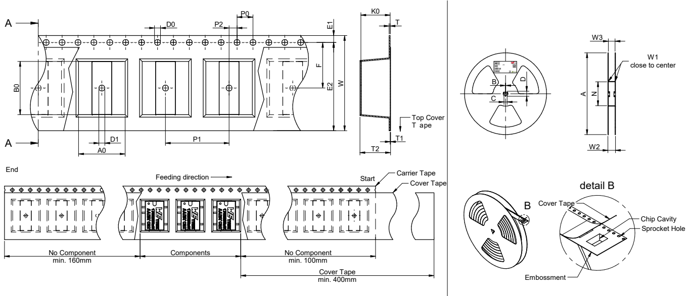
Figure 21: Packaging dimensions.
