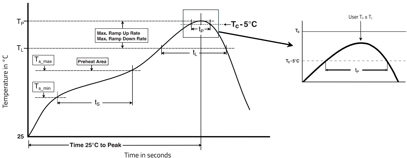
Figure 18: Solder profile.
