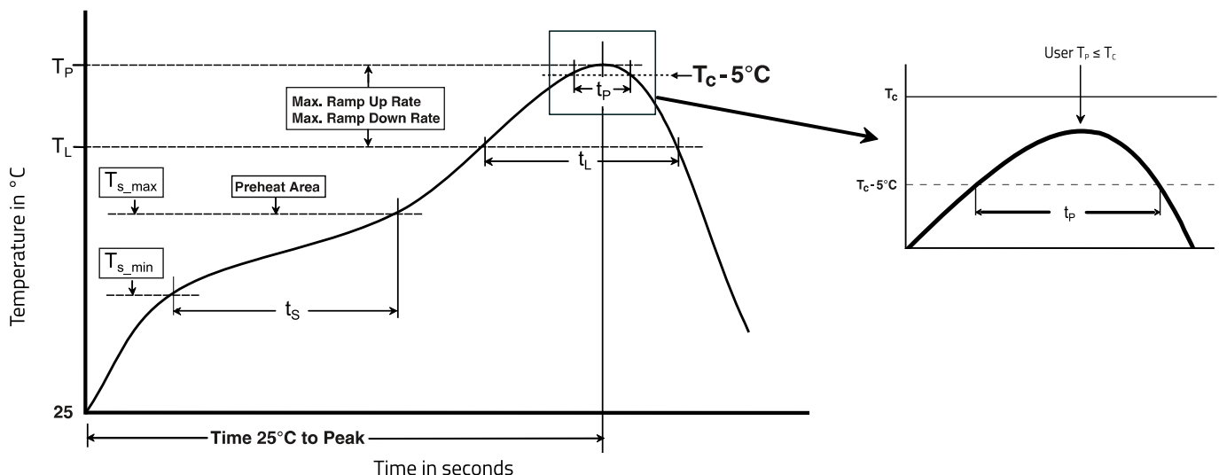
Figure 18: Solder profile.
