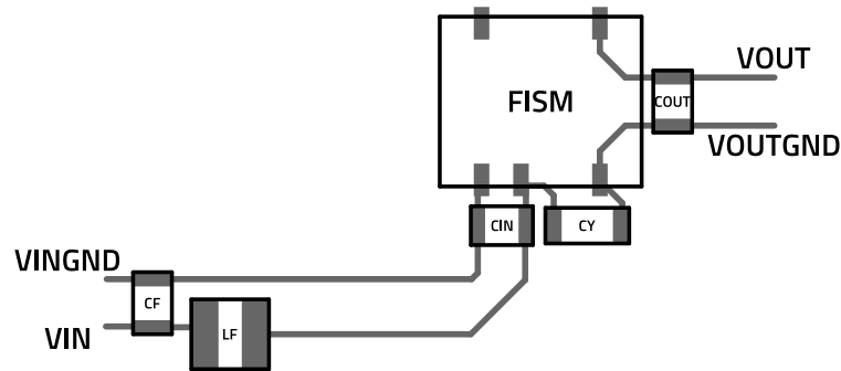
Figure 12: Layout recommendation.
