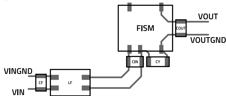
Figure 12: Layout recommendation.
