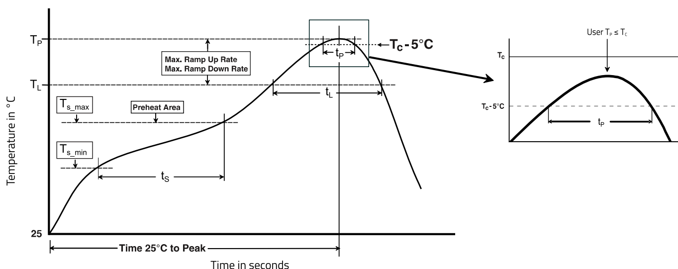
Figure 18: Solder profile.
