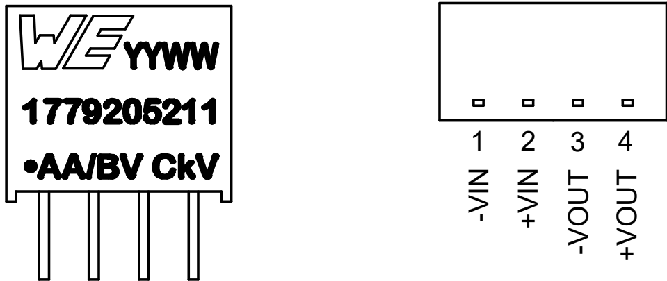
Figure 1: Pinout.
