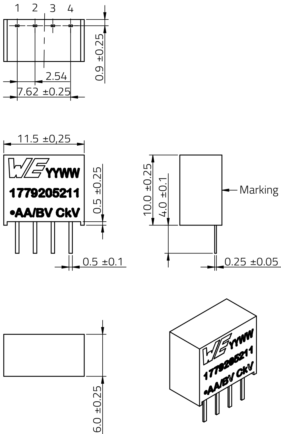
Figure 19: Component dimensions.
