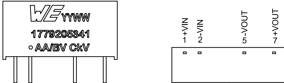
Figure 1: Pinout.
