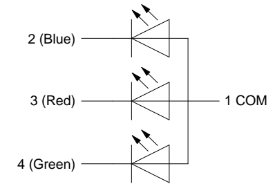
LED Schemaitc
