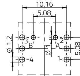
P.C.B. MOUNTING PLAN
