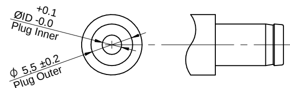
Recommended DC mate plug
