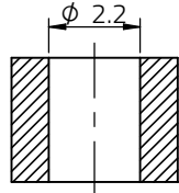
sectional drawing A-A
