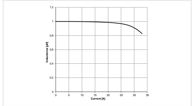
Typical Inductance vs. Current Characteristics: 7847227010
