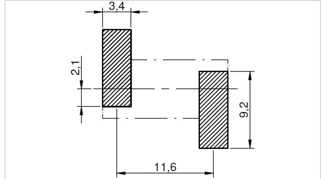
Recommended Land Pattern: [mm] 7847227010
