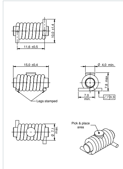
Dimensions: [mm] 7847227010
