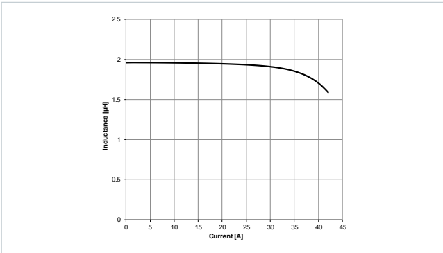
Typical Inductance vs. Current Characteristics: 7847229020
