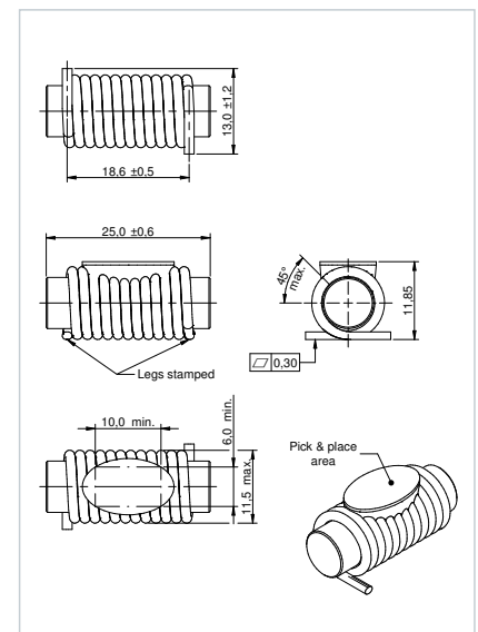
Dimensions: [mm] 7847232045
