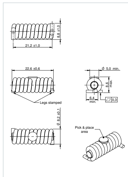
Dimensions: [mm] 7847239015
