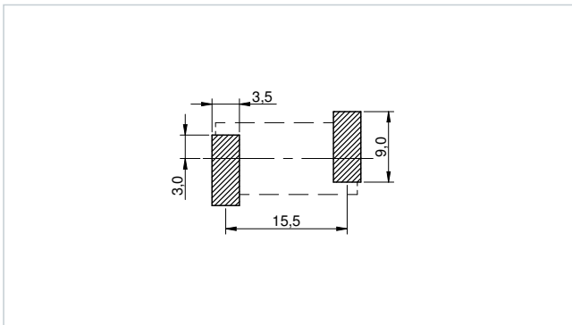
Recommended Land Pattern: [mm] 7847229020
