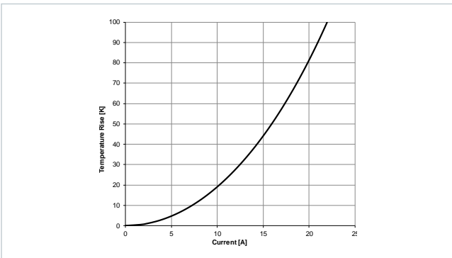
Typical Temperature Rise vs. Current Characteristics: 7847229020
