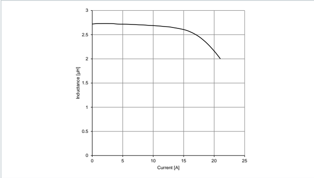
Typical Inductance vs. Current Characteristics: 7847227027
