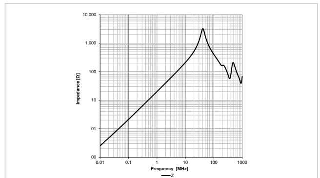
Typical Impedance Characteristics: 7847232045
