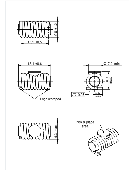
Dimensions: [mm] 7847229020
