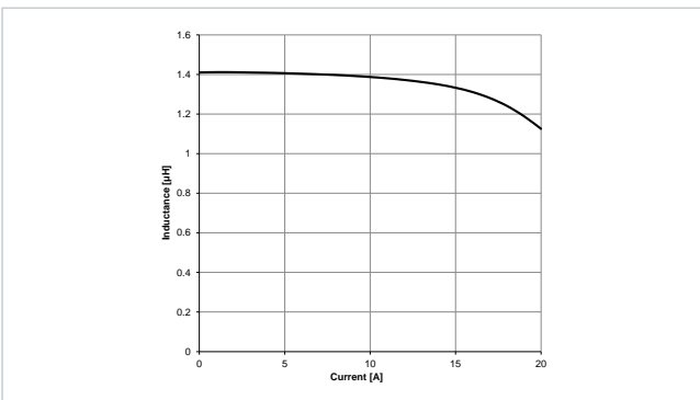
Typical Inductance vs. Current Characteristics: 7847239015
