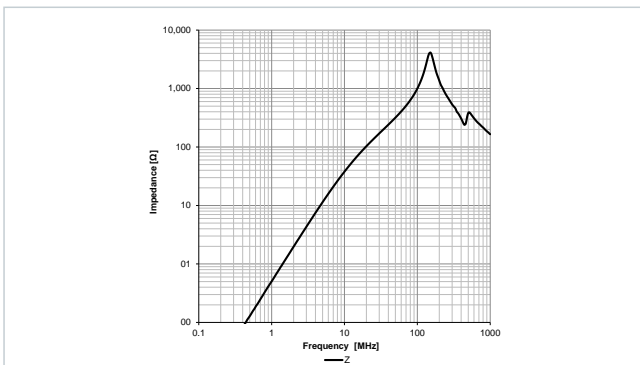
Typical Impedance Characteristics: 7847239015
