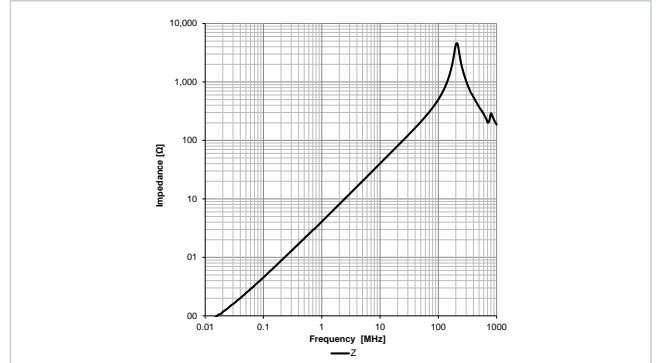
Typical Impedance Characteristics: 7847227010
