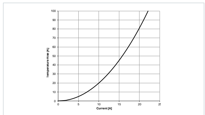
Typical Temperature Rise vs. Current Characteristics: 7847232045
