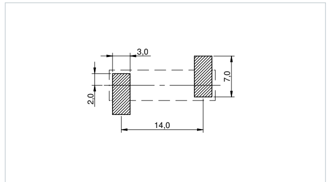
Recommended Land Pattern: [mm] 7847225100
