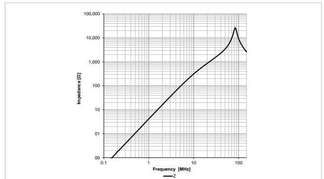
Typical Impedance Characteristics: 7847225100
