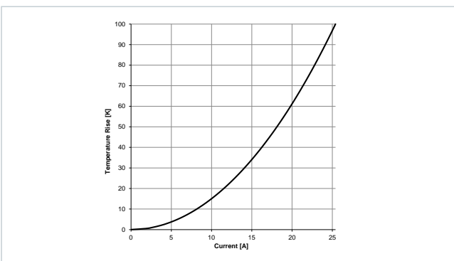
Typical Temperature Rise vs. Current Characteristics: 7847239015
