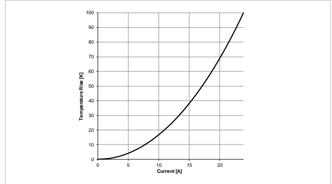
Typical Temperature Rise vs. Current Characteristics: 7847227010
