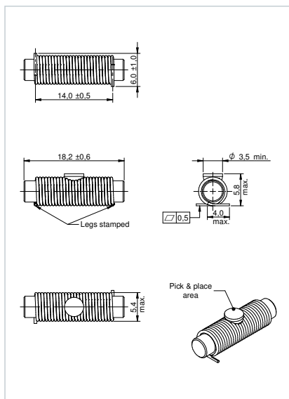
Dimensions: [mm] 7847225100
