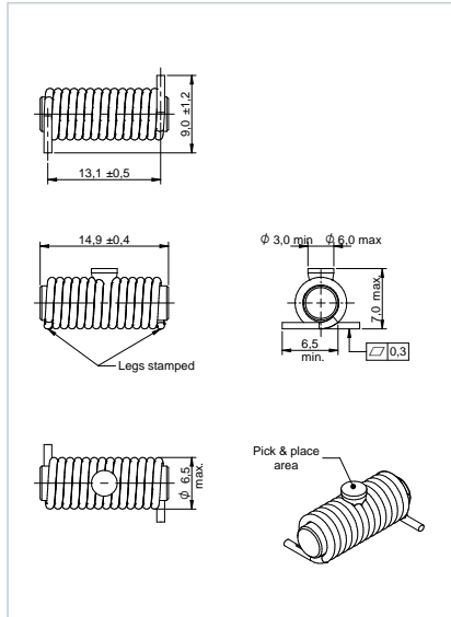
Dimensions: [mm] 7847227027
