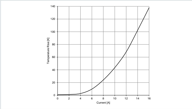
Typical Temperature Rise vs. Current Characteristics: 7847227027
