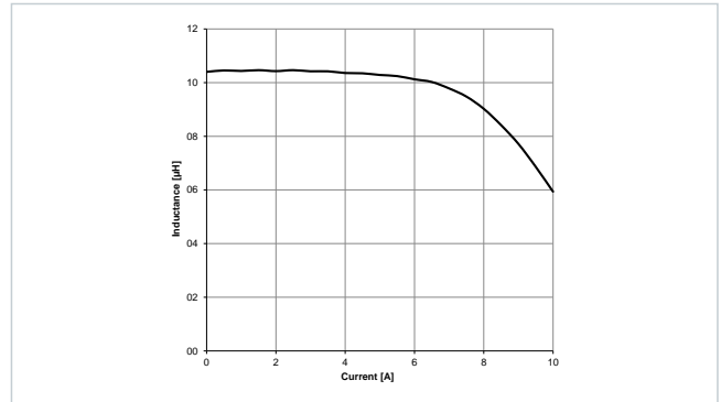
Typical Inductance vs. Current Characteristics: 7847225100
