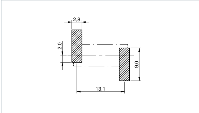
Recommended Land Pattern: [mm] 7847227027
