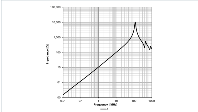
Typical Impedance Characteristics: 7847227027
