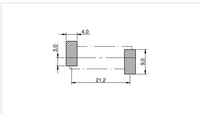
Recommended Land Pattern: [mm] 7847239015
