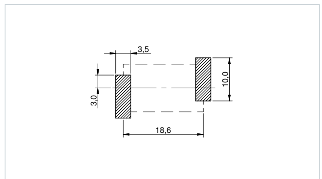
Recommended Land Pattern: [mm] 7847232045
