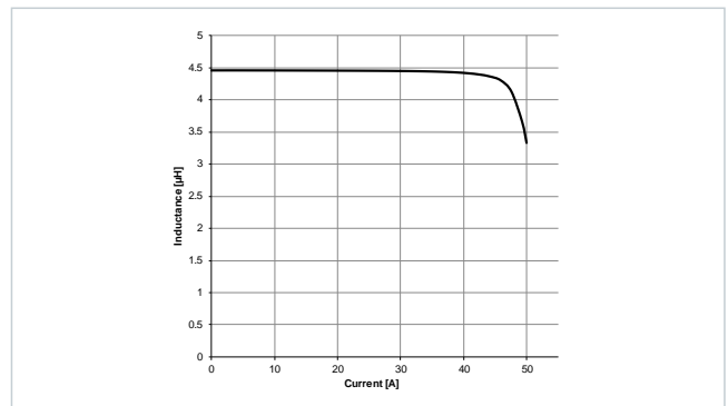
Typical Inductance vs. Current Characteristics: 7847232045
