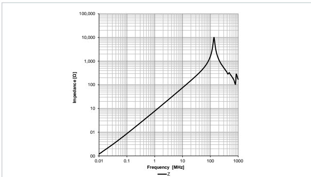
Typical Impedance Characteristics: 7847229020
