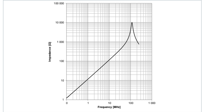
Typical Impedance Characteristics: 7847131020
