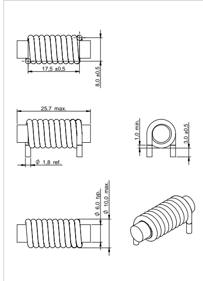
Dimensions: [mm] 7847131020
