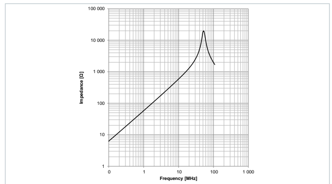
Typical Impedance Characteristics: 7847131100
