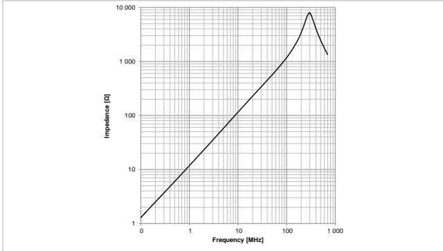
Typical Impedance Characteristics: 7847110020
