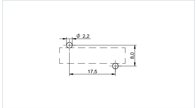
Recommended Hole Pattern: [mm] 7847131020
