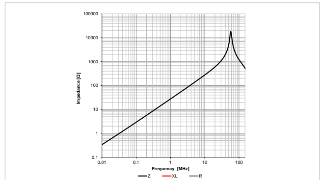
Typical Impedance Characteristics: 7847132060
