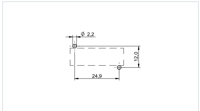
Recommended Hole Pattern: [mm] 7847132060
