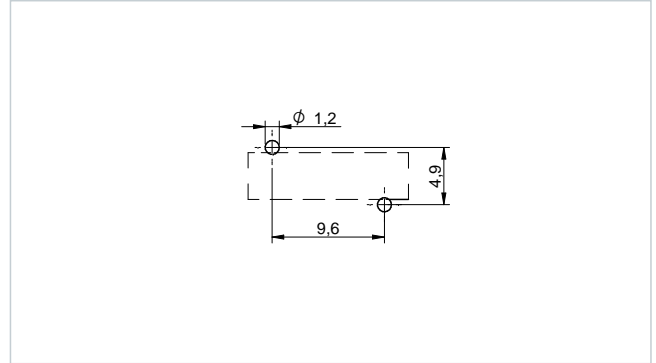
Recommended Hole Pattern: [mm] 7847111020
