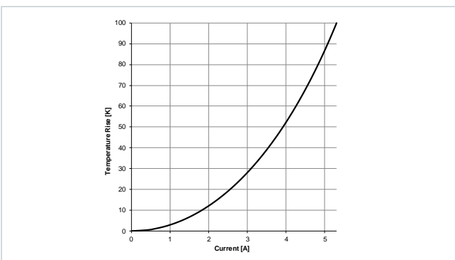
Typical Temperature Rise vs. Current Characteristics: 7847111100
