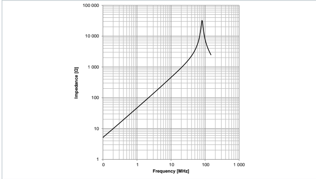
Typical Impedance Characteristics: 7847121100
