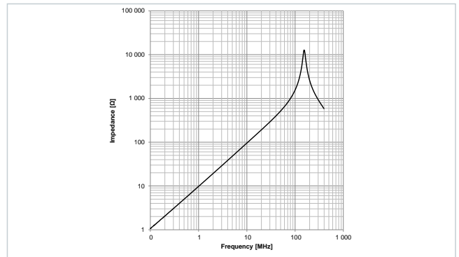
Typical Impedance Characteristics: 7847121020
