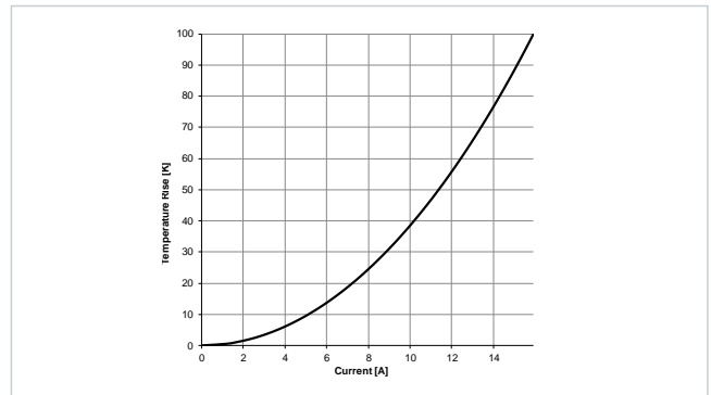
Typical Temperature Rise vs. Current Characteristics: 7847121020
