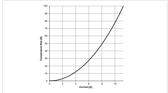
Typical Temperature Rise vs. Current Characteristics: 7847111020
