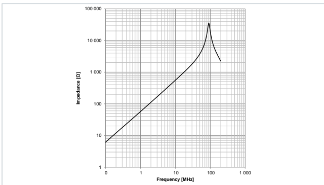
Typical Impedance Characteristics: 7847111100
