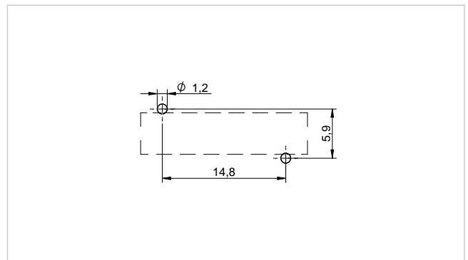
Recommended Hole Pattern: [mm] 7847121060
