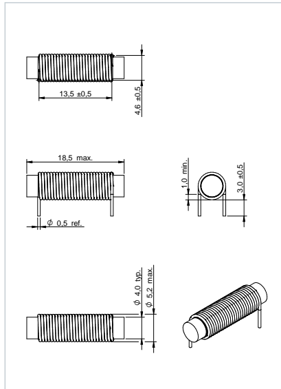
Dimensions: [mm] 7847111100
