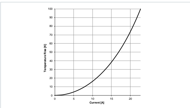
Typical Temperature Rise vs. Current Characteristics: 7847132100
