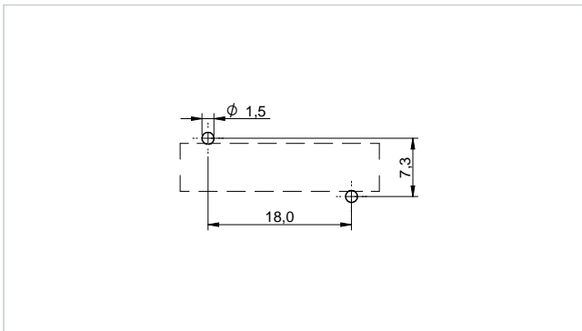
Recommended Hole Pattern: [mm] 7847131060
