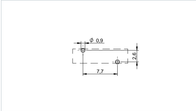
Recommended Hole Pattern: [mm] 7847110020
