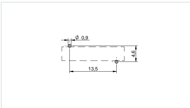
Recommended Hole Pattern: [mm] 7847111100
