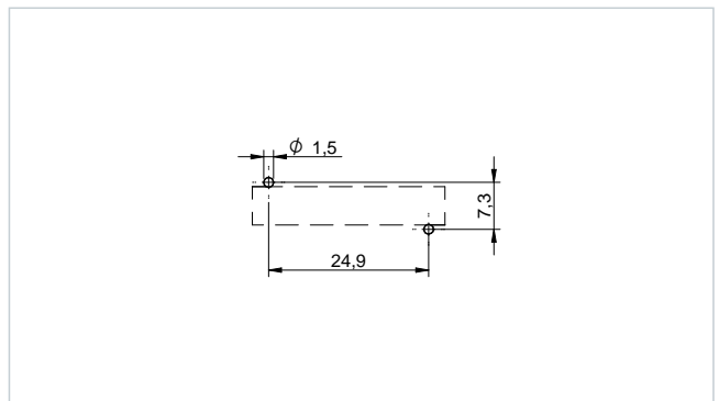
Recommended Hole Pattern: [mm] 7847131100
