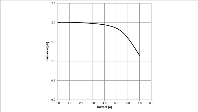
Typical Inductance vs. Current Characteristics: 7847110020
