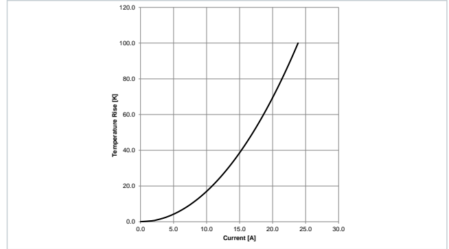
Typical Temperature Rise vs. Current Characteristics: 7847131020
