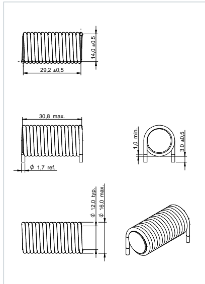
Dimensions: [mm] 7847132100
