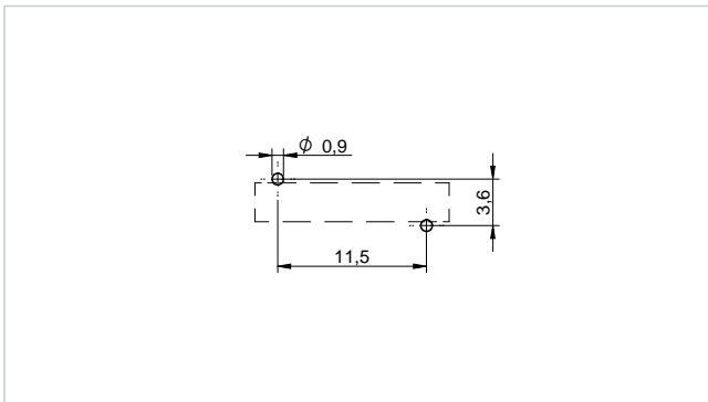
Recommended Hole Pattern: [mm] 7847120060
