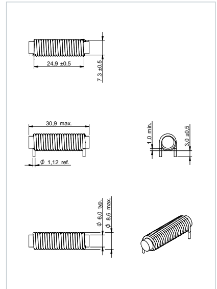
Dimensions: [mm] 7847131100
