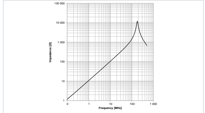
Typical Impedance Characteristics: 7847111020
