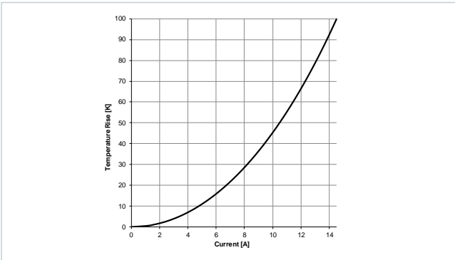
Typical Temperature Rise vs. Current Characteristics: 7847131060
