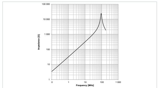
Typical Impedance Characteristics: 7847121060
