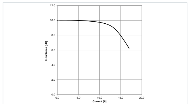
Typical Inductance vs. Current Characteristics: 7847131100
