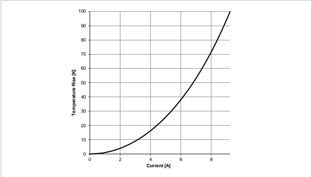
Typical Temperature Rise vs. Current Characteristics: 7847121100
