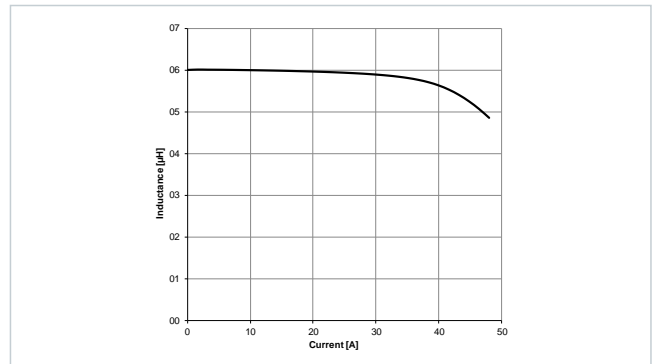
Typical Inductance vs. Current Characteristics: 7847132060
