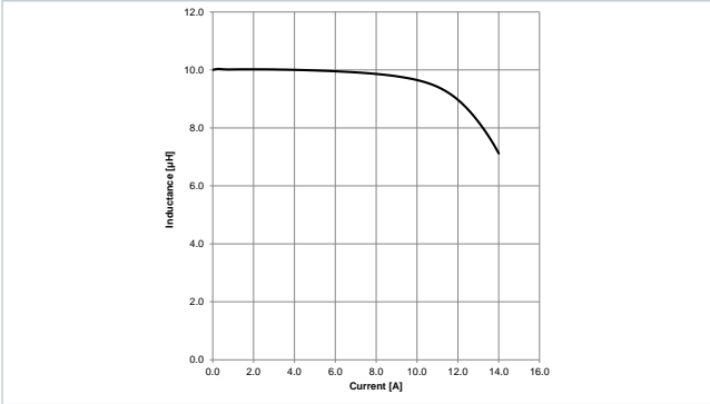
Typical Inductance vs. Current Characteristics: 7847121100
