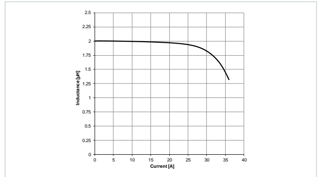
Typical Inductance vs. Current Characteristics: 7847121020
