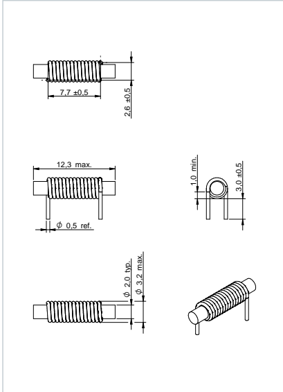
Dimensions: [mm] 7847110020
