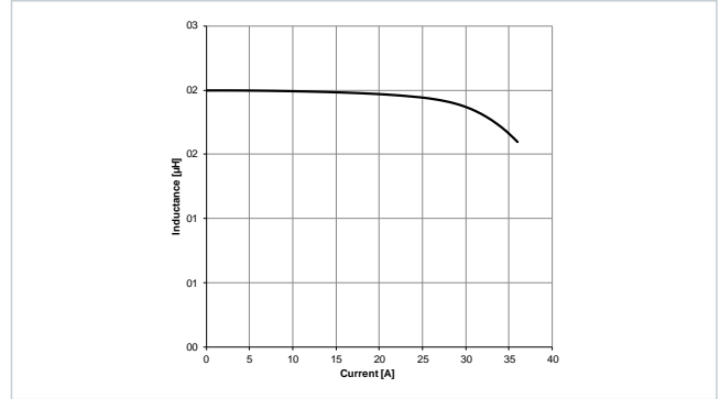
Typical Inductance vs. Current Characteristics: 7847131020
