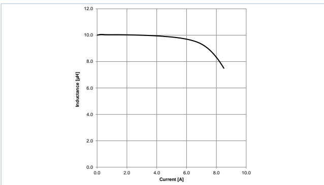
Typical Inductance vs. Current Characteristics: 7847111100
