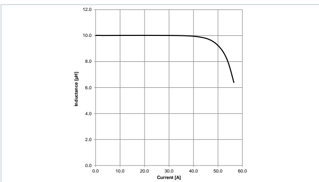
Typical Inductance vs. Current Characteristics: 7847132100
