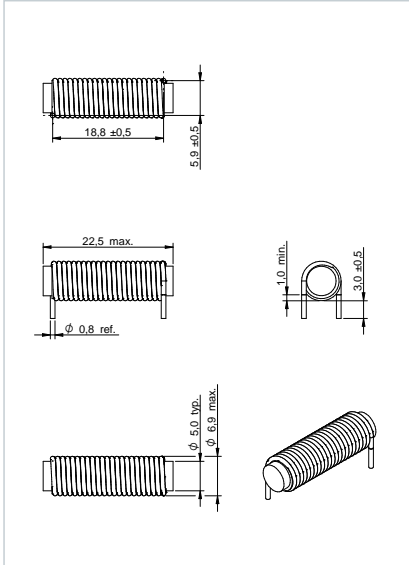
Dimensions: [mm] 7847121100
