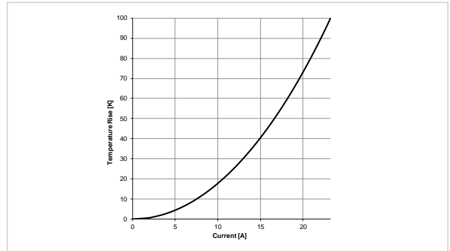
Typical Temperature Rise vs. Current Characteristics: 7847132060
