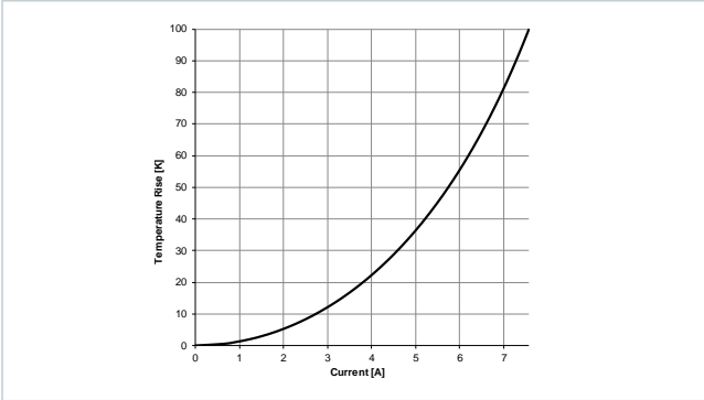
Typical Temperature Rise vs. Current Characteristics: 7847110020
