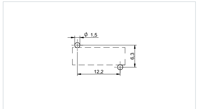
Recommended Hole Pattern: [mm] 7847121020
