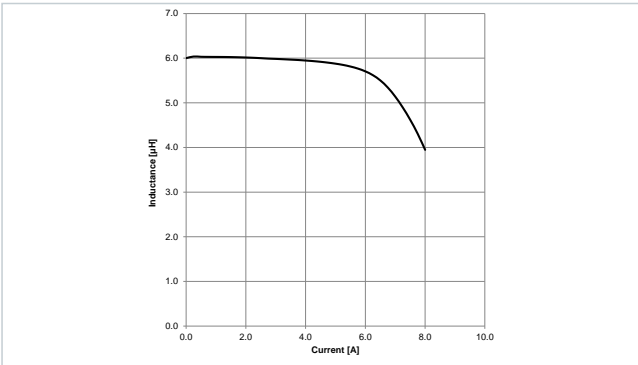
Typical Inductance vs. Current Characteristics: 7847120060
