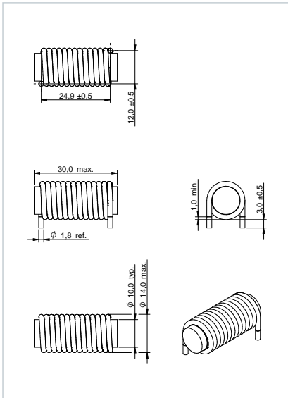
Dimensions: [mm] 7847132060
