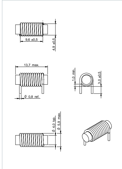
Dimensions: [mm] 7847111020
