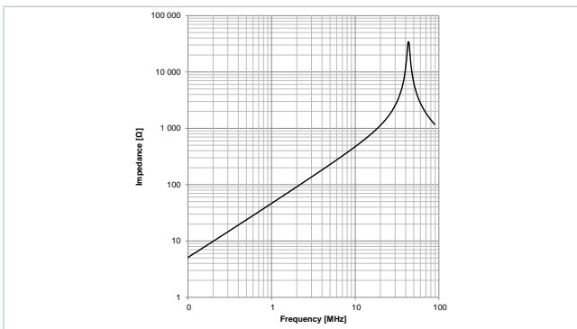
Typical Impedance Characteristics: 7847132100
