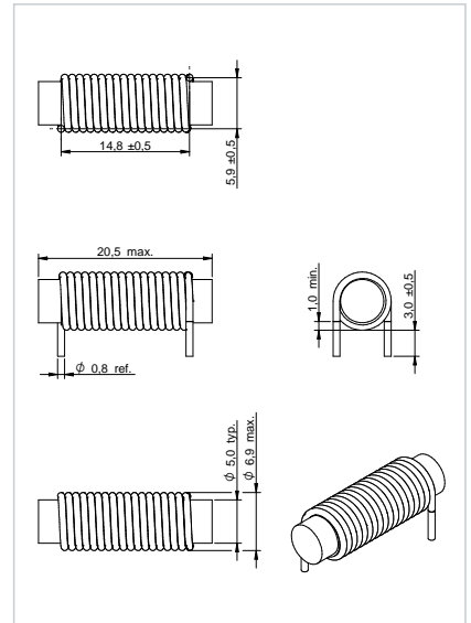
Dimensions: [mm] 7847121060
