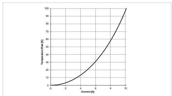
Typical Temperature Rise vs. Current Characteristics: 7847121060
