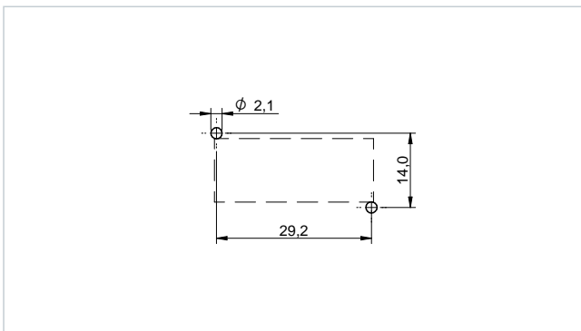
Recommended Hole Pattern: [mm] 7847132100
