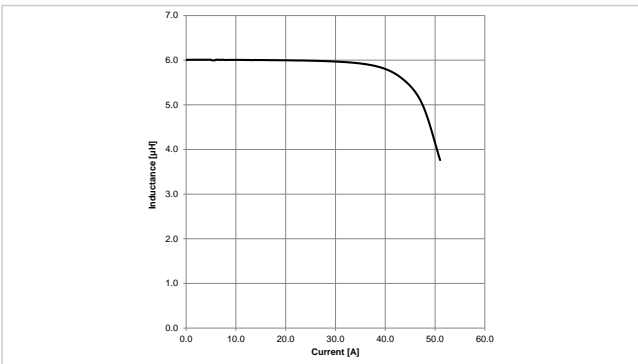
Typical Inductance vs. Current Characteristics: 7847131060
