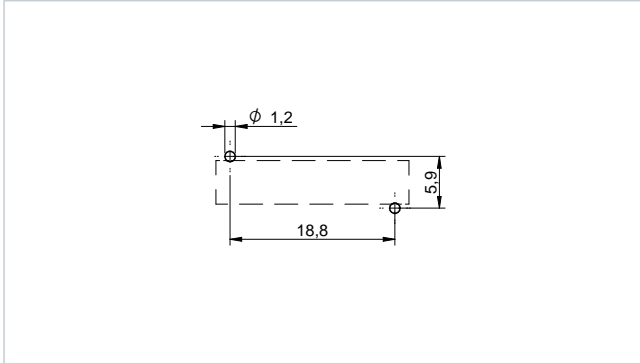
Recommended Hole Pattern: [mm] 7847121100
