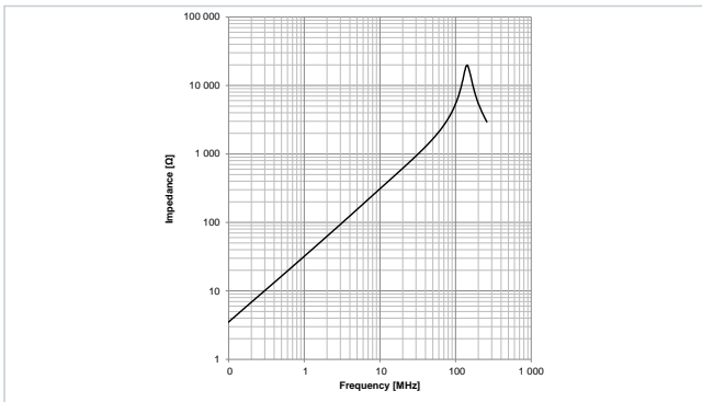
Typical Impedance Characteristics: 7847120060
