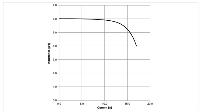
Typical Inductance vs. Current Characteristics: 7847121060
