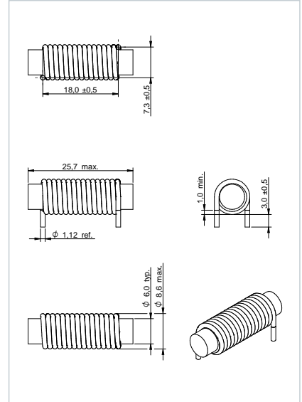
Dimensions: [mm] 7847131060
