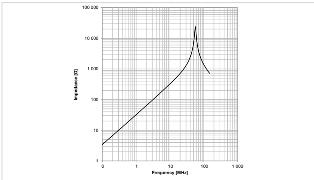
Typical Impedance Characteristics: 7847131060
