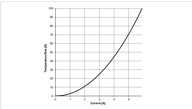
Typical Temperature Rise vs. Current Characteristics: 7847120060
