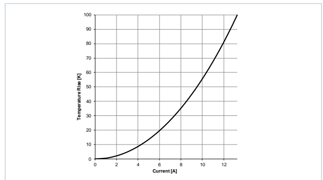
Typical Temperature Rise vs. Current Characteristics: 7847131100
