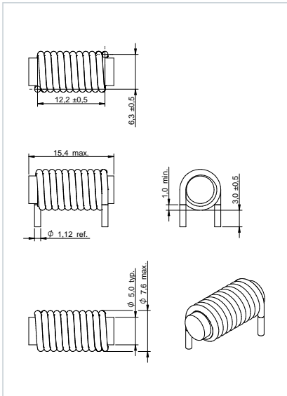
Dimensions: [mm] 7847121020
