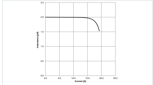
Typical Inductance vs. Current Characteristics: 7847111020
