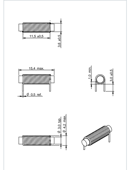
Dimensions: [mm] 7847120060
