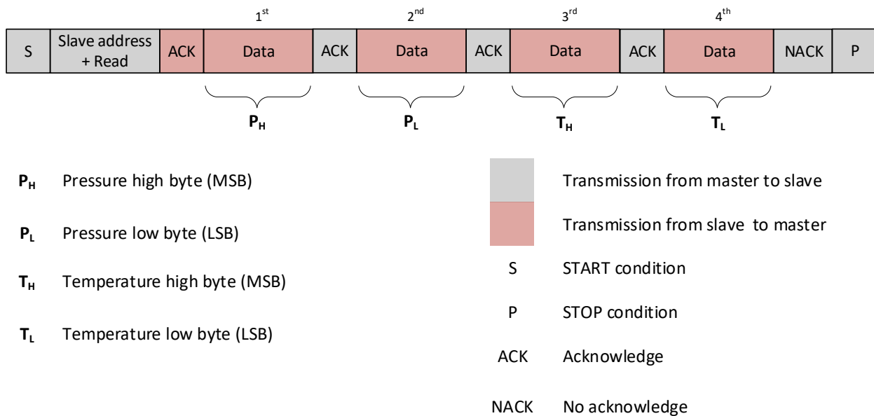
Host controller reading multiple data bytes from the sensor (slave)
