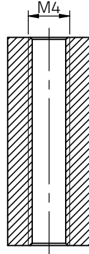
sectional drawing A-A
